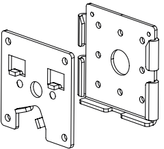
Staffa scorrevole interasse 48 box Sliding bracket center-to-center 48 box
